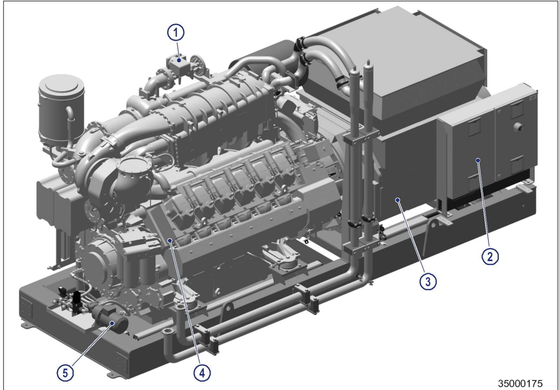
Figure 3: Engine-generator set - Engine end
