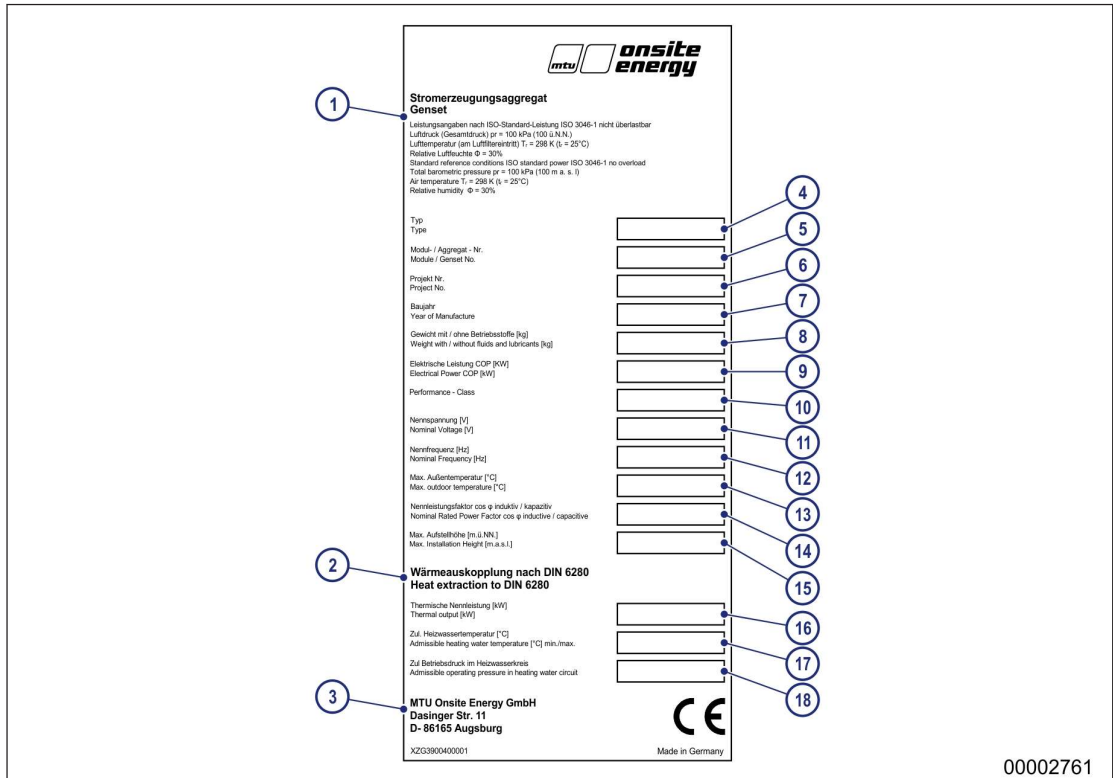
Figure 2: Nameplate of engine-generator set
